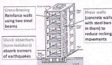
Earthquake Resistant Building
